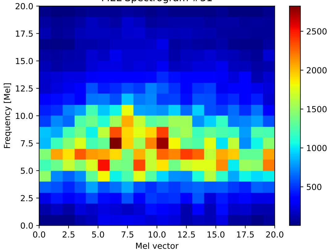
MEL Spectrogram #31
